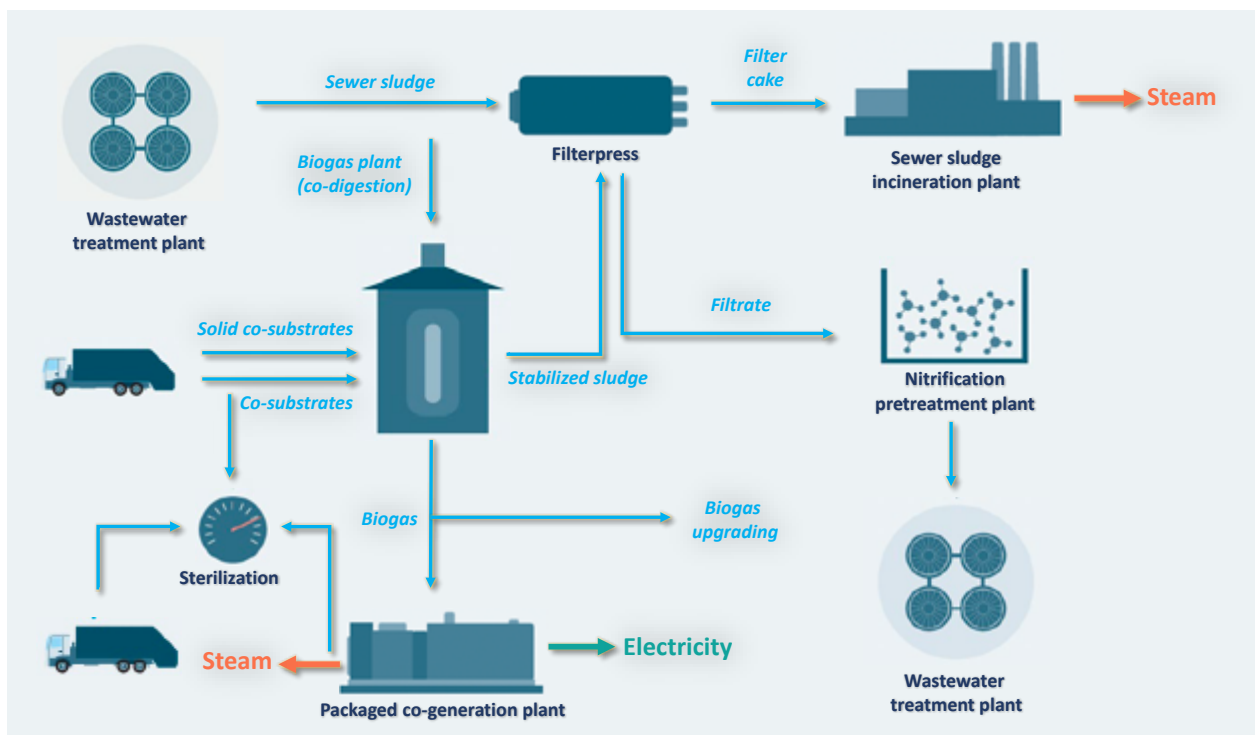
FIGURE A4.7: INTEGRATED SYSTEM OF SLUDGE FROM A WASTEWATER TREATMENT PLANT, INDUSTRIEPARK HÖCHST
